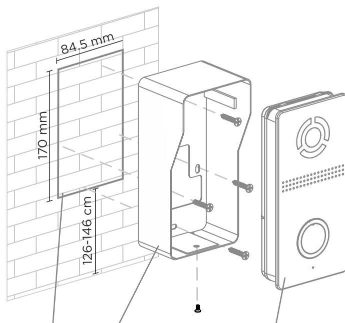
Niche Surface Bracket with Sun & Rain Cover Outdoor Panel
