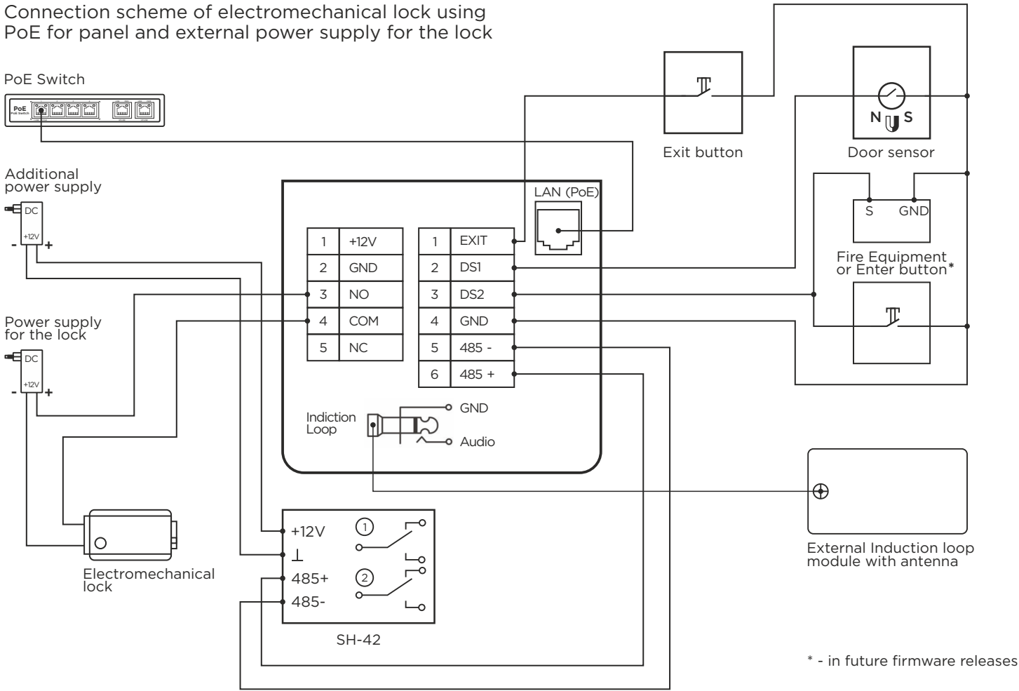
Connection scheme of electromagnetic lock using PoE for panel and external power supply for the lock
