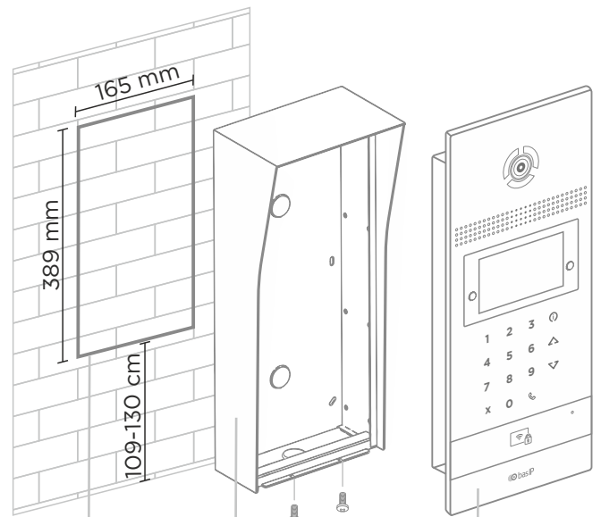
Mounting area
