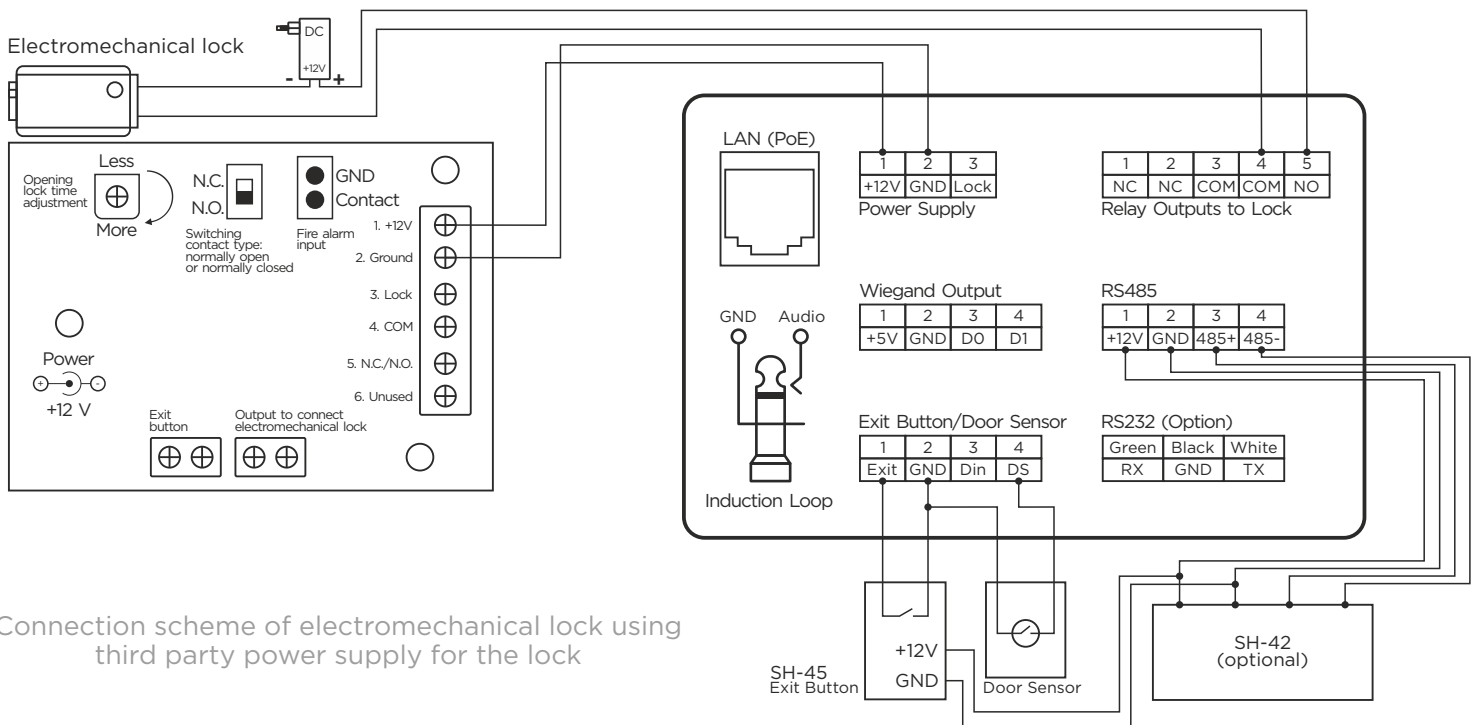
Connection scheme of electromechanical lock using uninterruptible power supply UPS-DP/F
